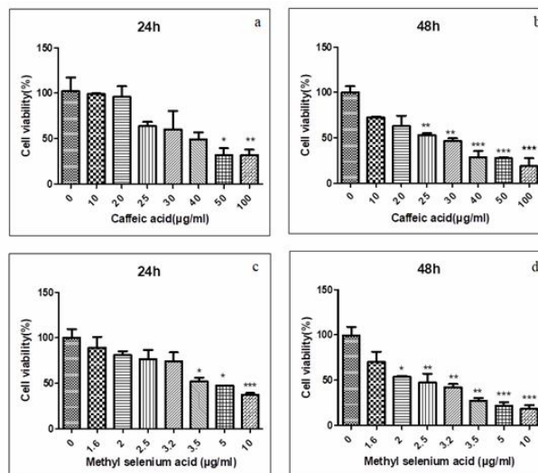
Fig. 1. Survival percentage of MDA-MB 231 cells treated with different concentrations of CA (0-100 \mu g ml -1 ) after (a) 24 h and (b) 48 h. Survival percentage of MDA-MB 231 cells treated with different concentrations of MSA (0-10 \mu g ml -1 ) after (c) 24 h and (d) 48 h. Cell viability was analyzed by MTT assay. Data are reported as means \pm SD. (*P < 0.1, **P < 0.01, ***P < 0.001; ANOVA test, TUKEY test).
